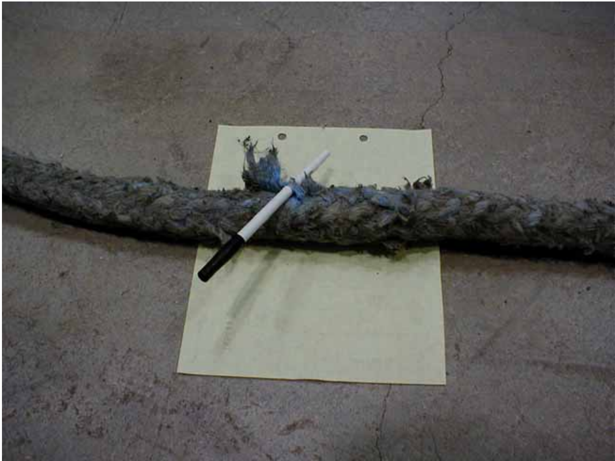
Figure R9. Severe abrasion in a section of 7/8-inch ASB synthetic winch line. Pen is inserted underneath the intact remnants of a strand. Manufacturer's recommendation is to retire a rope or cut and re-splice the remaining rope when 2 or more adjacent strands are cut.
